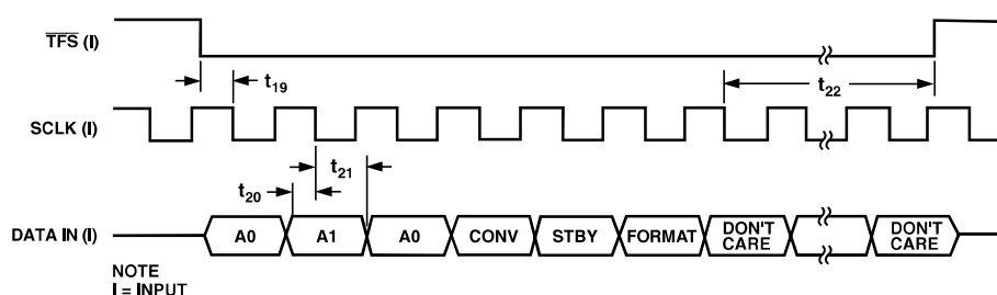
Figure 4. Serial Mode Write Operation
