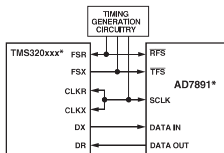
Figure 11. AD7891 to TMS320xxx Serial Interface
